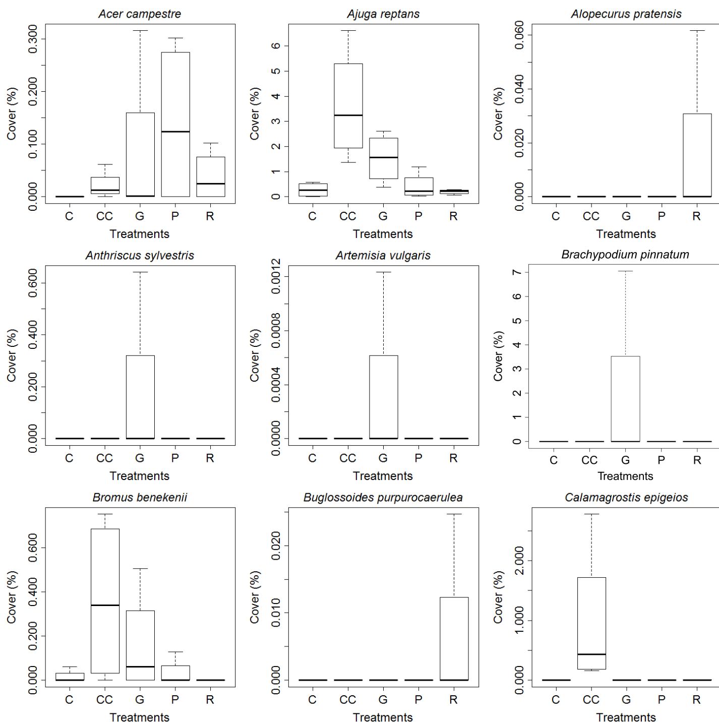
Fig. A3 Boxplots of the cover of the registered understory species in the different treatments, on plot level. C = control, CC = clear-cutting, G = gap-cutting, P = preparation cutting, R = retention tree group. Scaling of the different species is not uniform.
